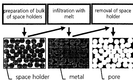
Figure 1: process for making porous metal sponges
