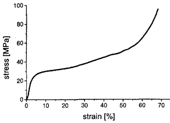
Figure 5: compression test on an Al sponge of density 1180 kg/m 3
