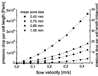
Figure 6: pressure drop in an aluminium sponge
