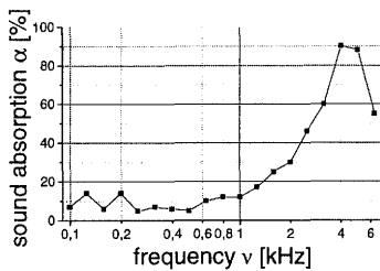
Figure 7: sound absorption curves measured on aluminium sponges
