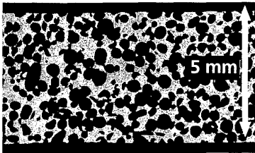
Figure 3: pore structure of an aluminium sponge.
