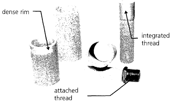
Figure 8: silencers made of aluminium sponge (all except the lying sample are closed on one side)
